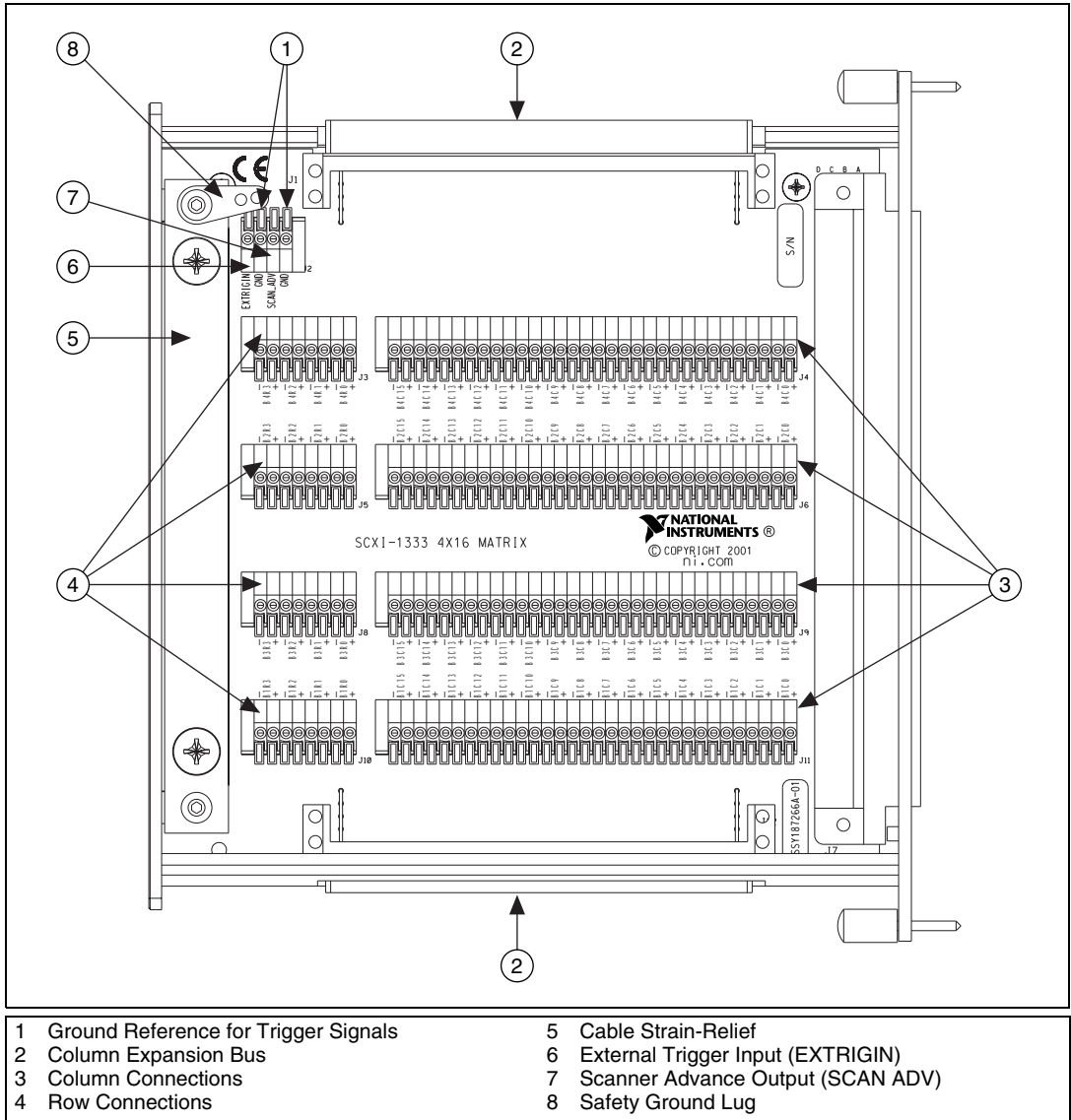
Figure 2-2. Terminal Block Example (SCXI-1333)
